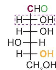
D-Glucose
