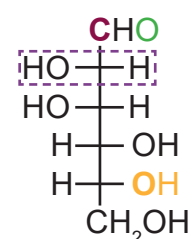
D-Mannose
