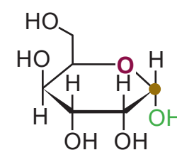
\alpha -D-Glucose
