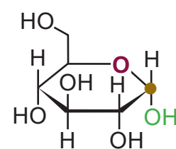
\alpha -D-(+)-Glucose
