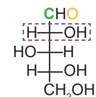
D-Xylose
